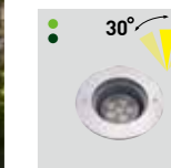
HBD-D075 W173xD173xH203mm 9.1W 3000K 570lm
