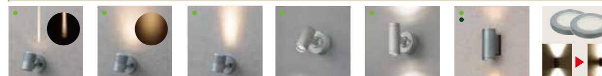
HBB-008D W80xD125xH88mm 4.8W 3000K 16lm HBB-009D W80xD125xH88mm 4.8W 3000K 185lm HBB-010D W80xD125xH88mm 4.8W 3000K 154lm HBA-D06S W55xD75xH68mm 1.1W 3000K 85lm HBA-D07S W55xD75xH79mm 2.2W 3000K 105lm HBA-D11L W80xD137xH180mm 21.0W 3000K 1507lm DIFFUSER LENS For HBA-D11L HBB-D11L W160xD270xH268mm 31.5W 3000K 2000lm
