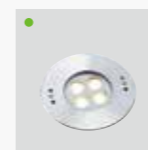
HHA-D07S W135xD135xH123mm 9.0W 3000K 500lm
