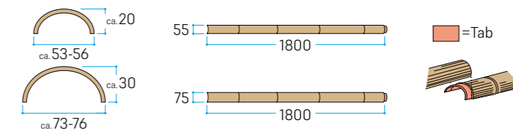
Cross bars
