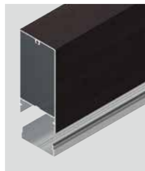
Size in mm 50x100xL3650 t: 1.3 mm
