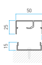
Size in mm 50x25xL4000 t: 1.2 mm
